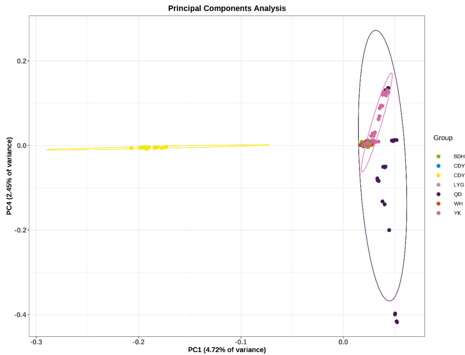
Figure 3. Principal component analysis. Each point indicates an individual and different colors indicate different groups.
